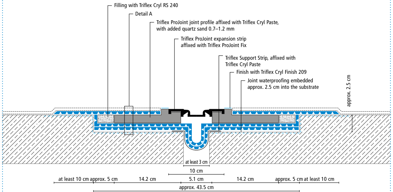
Drawing no.: ProJoint+-1561
