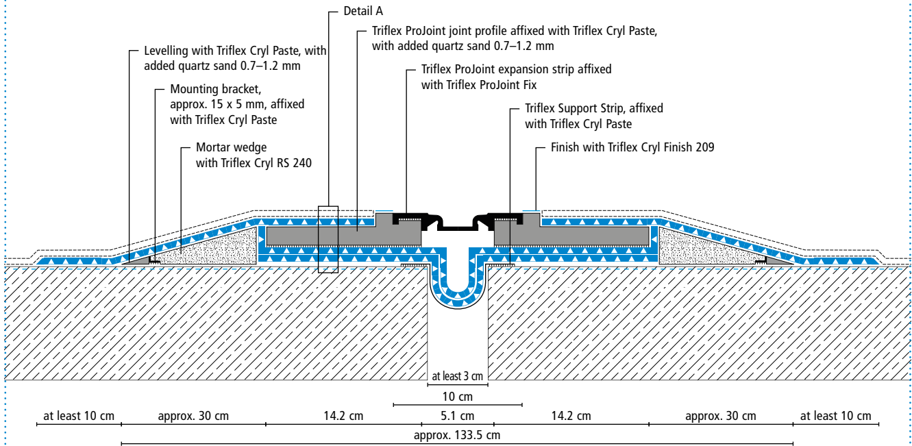
Drawing no.: ProJoint+-1562
