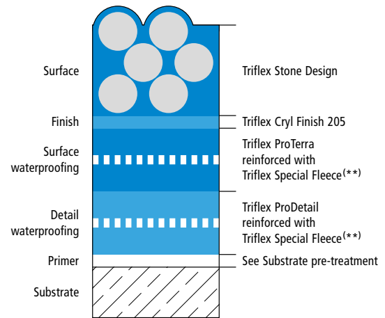
System build-up – Detail B
