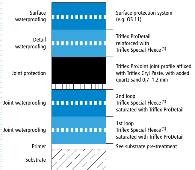
System build-up – Detail A
