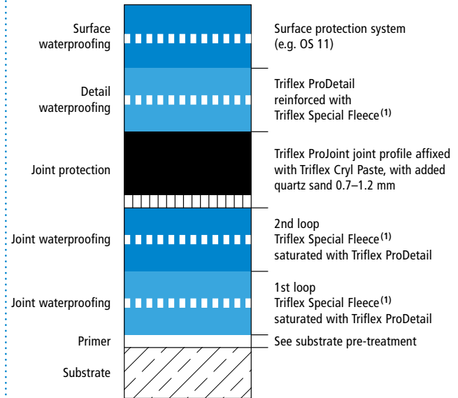
System build-up – Detail A
